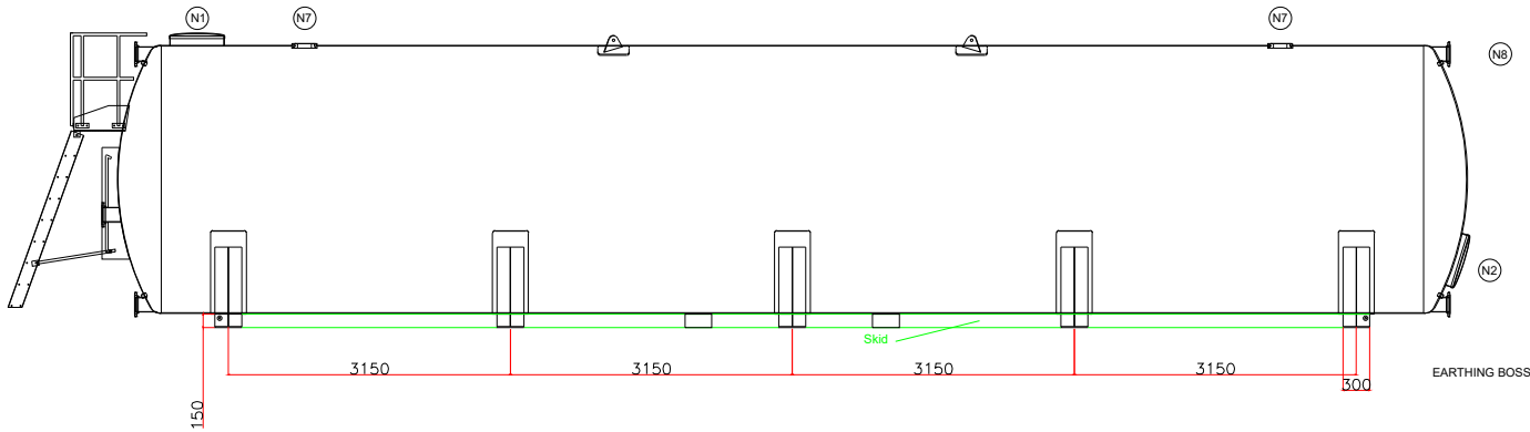
ELEVATION VIEW
